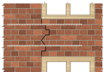
Crack stitching
